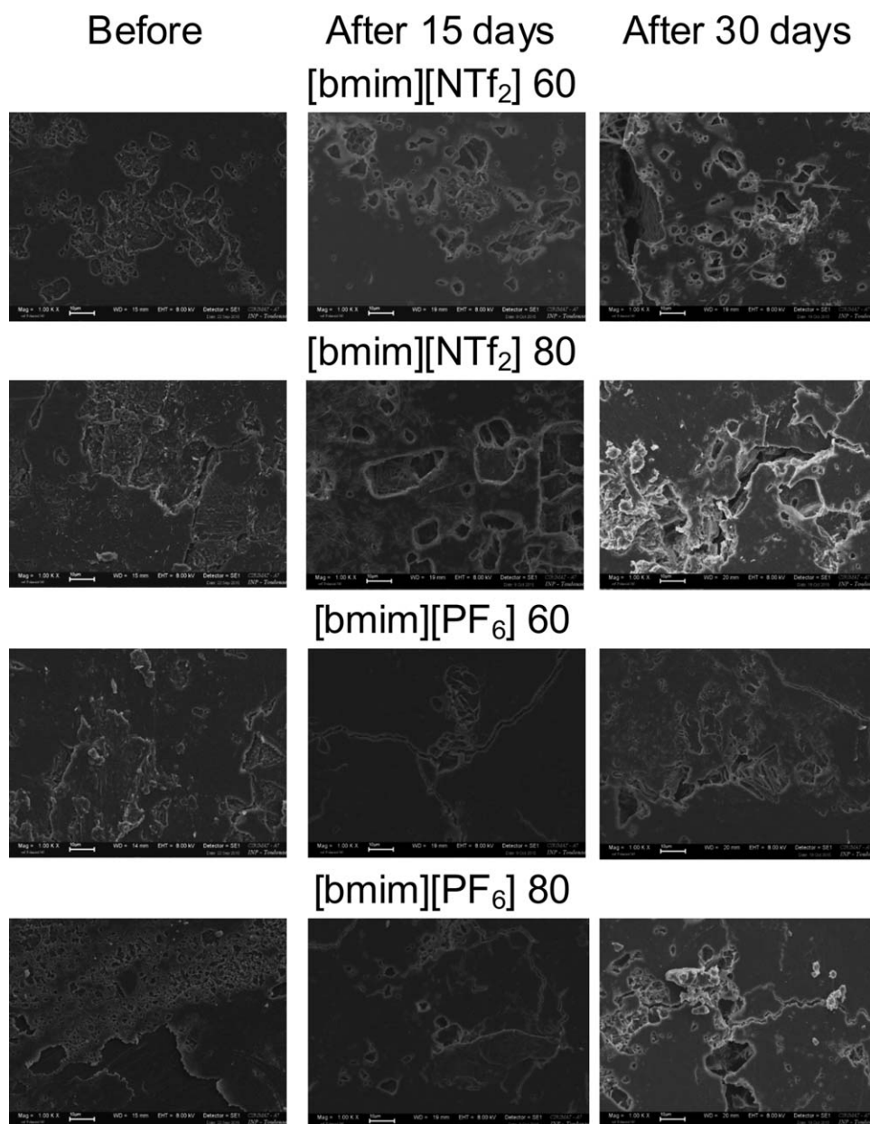
Figure 14. SEM micrographs showing the microstructure of the PCL tablets before and after 2 and 4 weeks of degradation test in PBS solution at 37 °C and pH 7.4 (scale bar corresponds to 10 \mu m).
